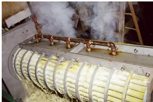
STEAM INJECTION IN TWIN SCREW PRESS
